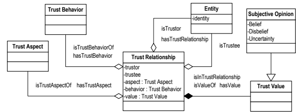
Figure 5. Trust basic UML model
